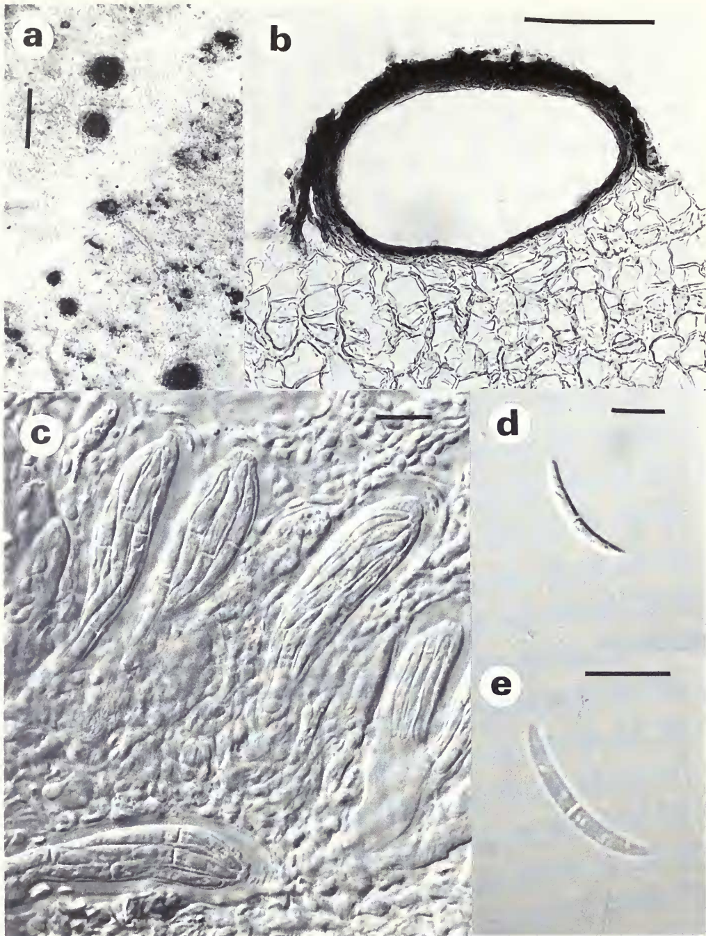
Fig. 3 Leptorhaphis atomaria (Ach.) Szat. (H-ACH 795a-lectotype) (a) Surface view of ascomata; scale = 500 \mu m; (b) Vertical section of ascoma, showing exciple extending below ascoma; scale = 100 \mu m; (c) Asci, ascospores and pseudoparaphyses; (d), (e) Ascospores; scale = 10 \mu m.
